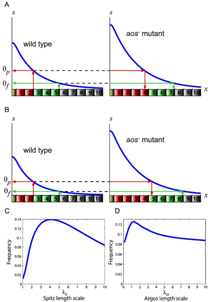
Fig. 3. Parameter screen based on aos - mutant data. (A, B) In wild type embryos, otd is expressed in two cell rows from the midline (red cells, left-hand panel), whereas FasIII is expressed in five cell rows (green and red cells, left-hand panel). We use the modeled Spitz profile to calculate \sigma_i , the amount of EGFR signal received by cell i . We then estimate the threshold signal level required for pnt (and hence otd ) expression and denote this \theta_p . Similarly, we calculate \theta_f , the threshold signal level required for FasIII expression. We then use these threshold values to determine the predicted range of otd and FasIII expression in the aos - mutant (right-hand panel). (A) Calculation performed for a “successful” parameter set: \lambda_s = 3 , \lambda_a = 5 , \mu = 3 , \nu = 1 . Note that the expansions depicted in the Argos mutant are consistent with the literature data. (B) Calculation performed for an “unsuccessful” parameter set: \lambda_s = 3 , \lambda_a = 5 , \mu = 5 , \nu = 1 . Note that the expansions depicted in the Argos mutant here are inconsistent with the literature data. (C, D) Distributions of length scales for all parameter sets that are “successful” in fitting the aos - mutant data.
