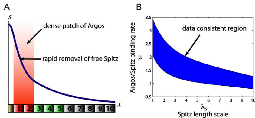
Fig. 5. Simplified model with immobile, localized, Argos. (A) Typical Spitz profile depicting the mode of action of localized Argos. Note the rapid decline in the Spitz profile in the region occupied by Argos. (B) Region of parameter space consistent with the aos^- data.
